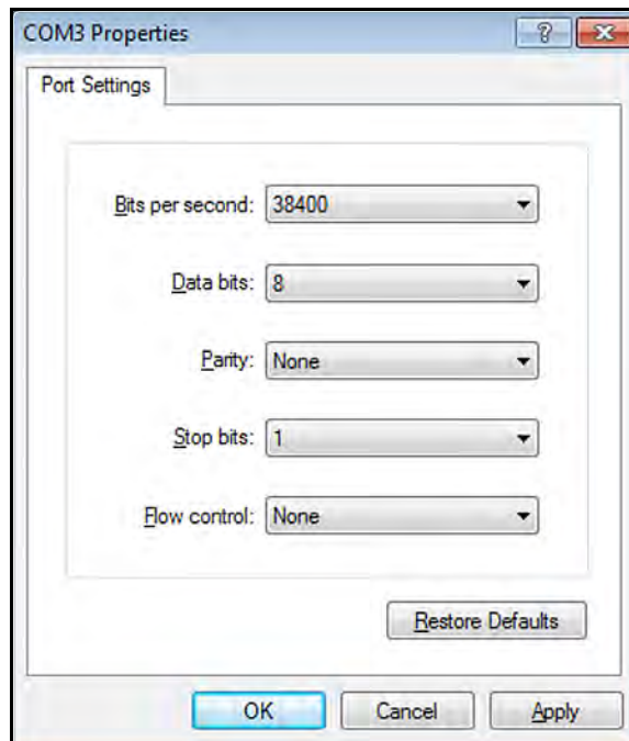
Figure 13: COM Properties
