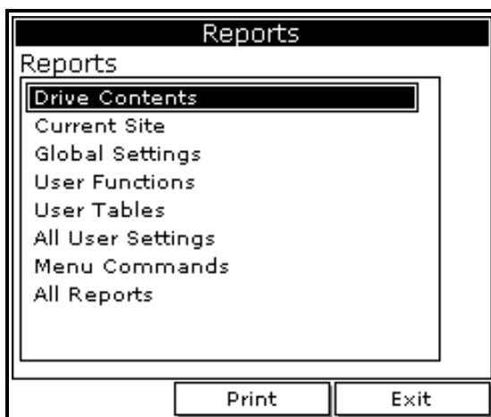
Figure 59: Reports Window
