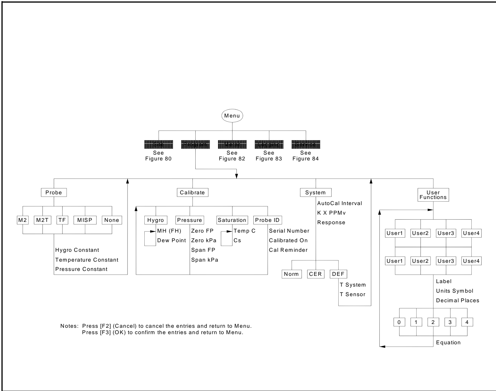
Figure 81: Program Menu
